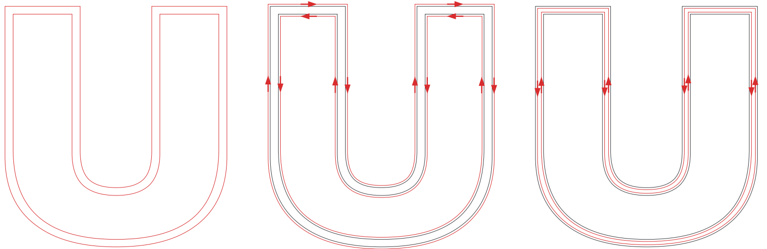
Lateral offset correct
